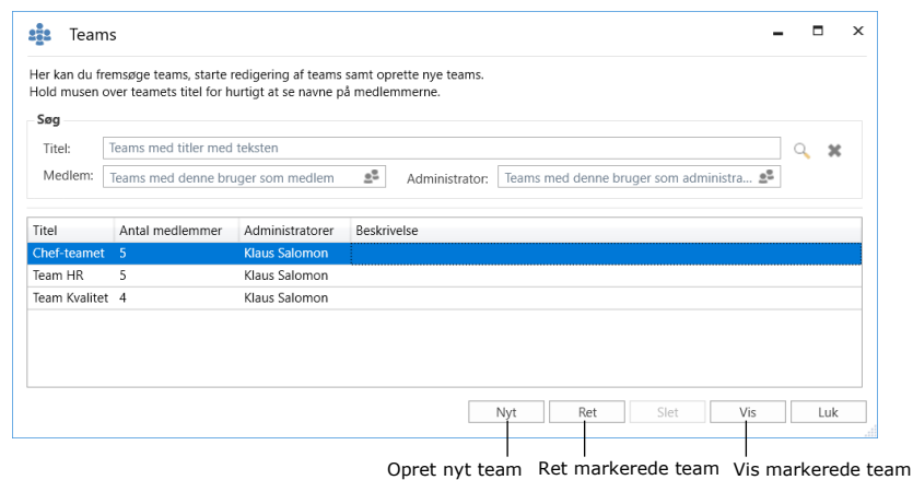
Figur 104: Dialogen "Teams"
